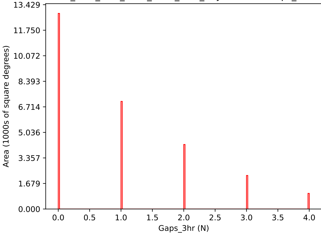
ddf_acor_sf15_lsf30_lsr20_v3.4_10yrs i band: Gaps_3hr
