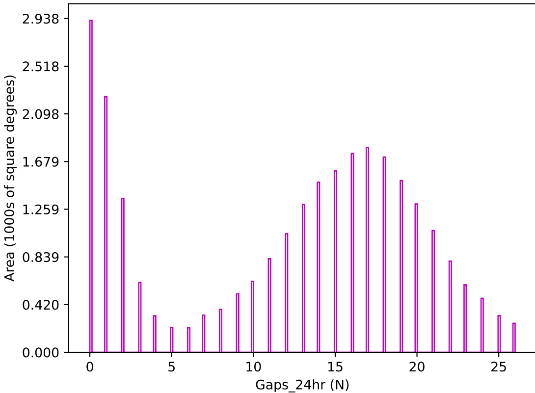
ddf_acor_sf15_lsf30_lsr20_v3.4_10yrs z band: Gaps_24hr
