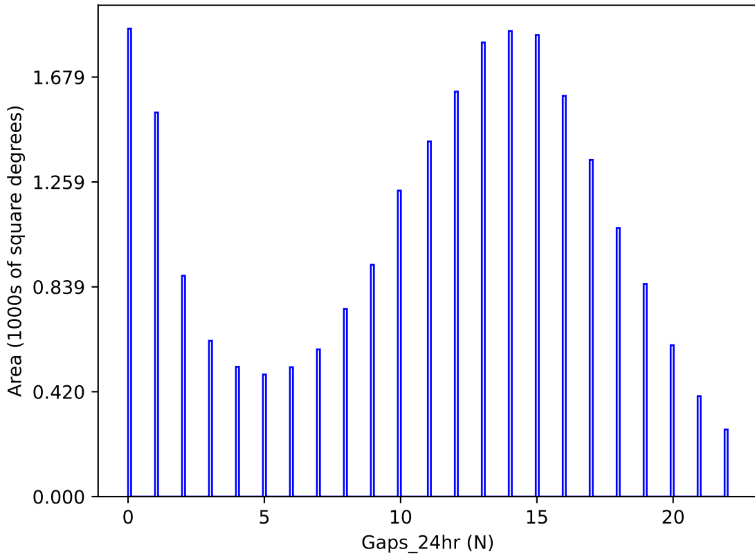
ddf_acor_sf15_lsf30_lsr20_v3.4_10yrs y band: Gaps_24hr
