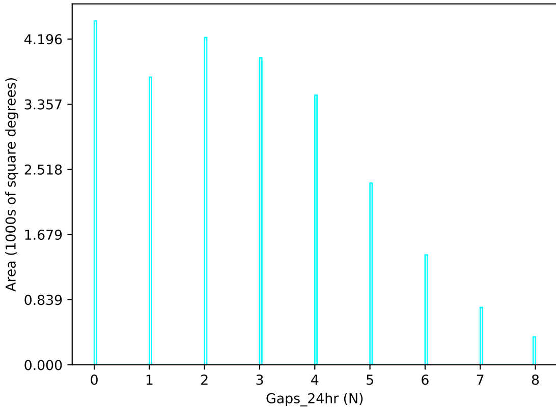
ddf_acor_sf15_lsf30_lsr20_v3.4_10yrs u band: Gaps_24hr
