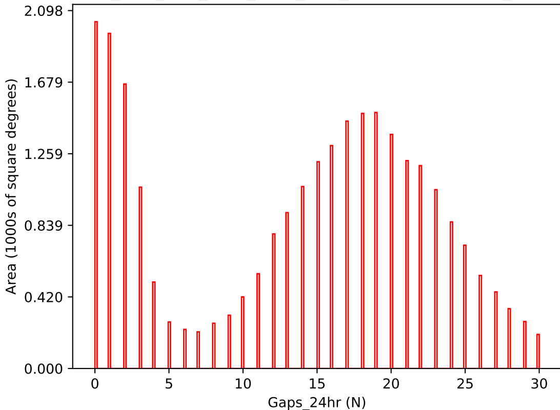
ddf_acor_sf15_lsf30_lsr20_v3.4_10yrs i band: Gaps_24hr
