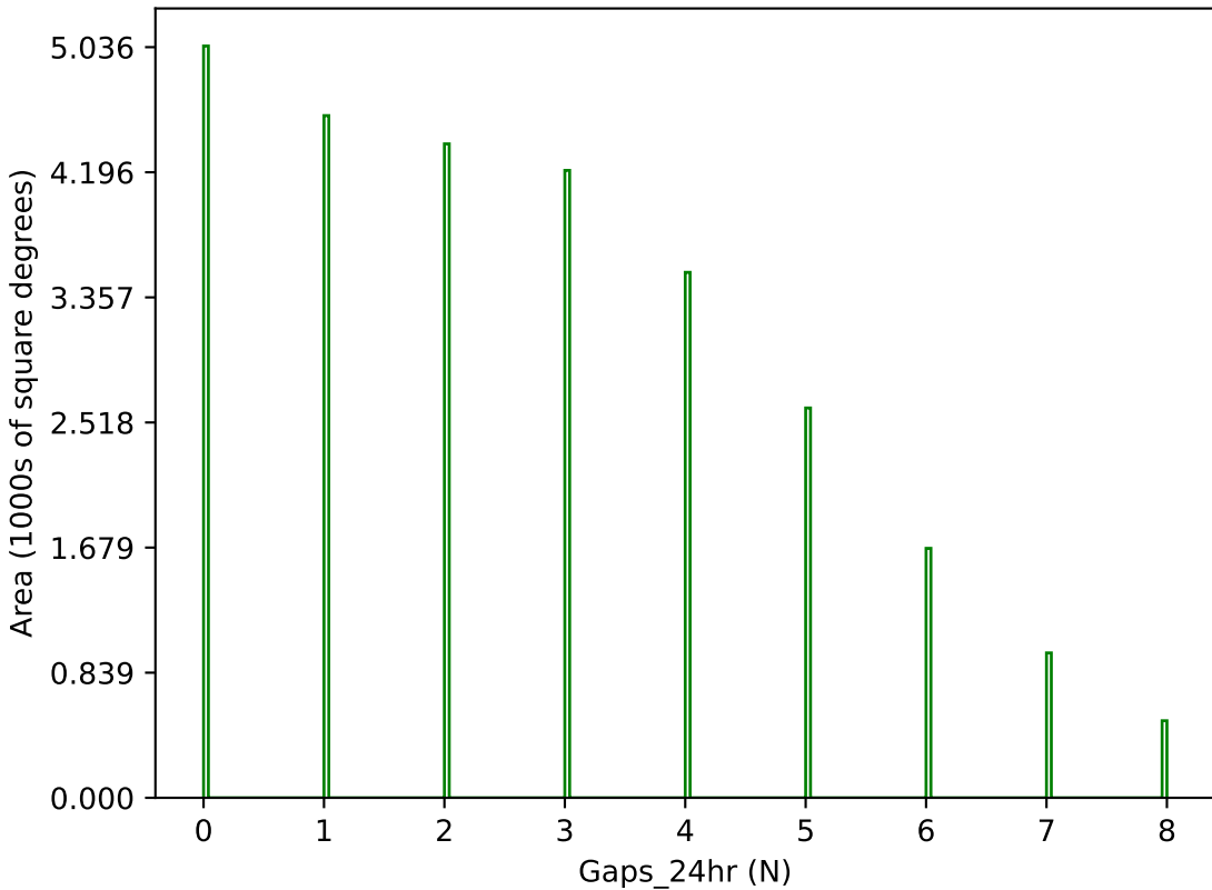
ddf_acor_sf15_lsf30_lsr20_v3.4_10yrs g band: Gaps_24hr
