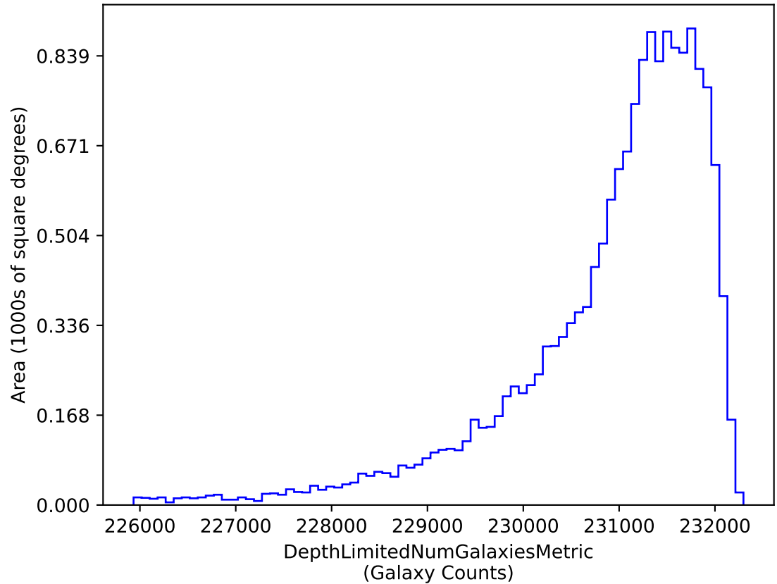
ddf_acor_sf15_lsf30_lsr20_v3.4_10yrs i band galaxies non-DD: DepthLimitedNumGalaxiesMetric
