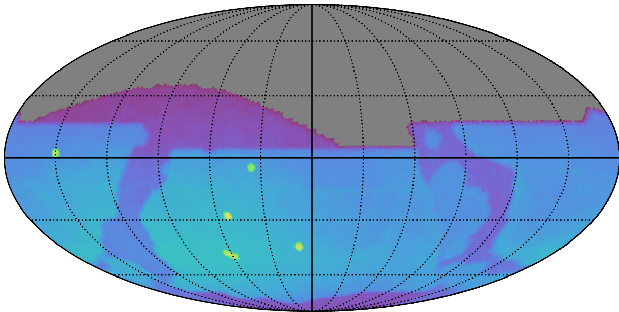
ddf_acor_sf15_lsf30_lsr20_v3.4_10yrs : Brown Dwarf, L7
