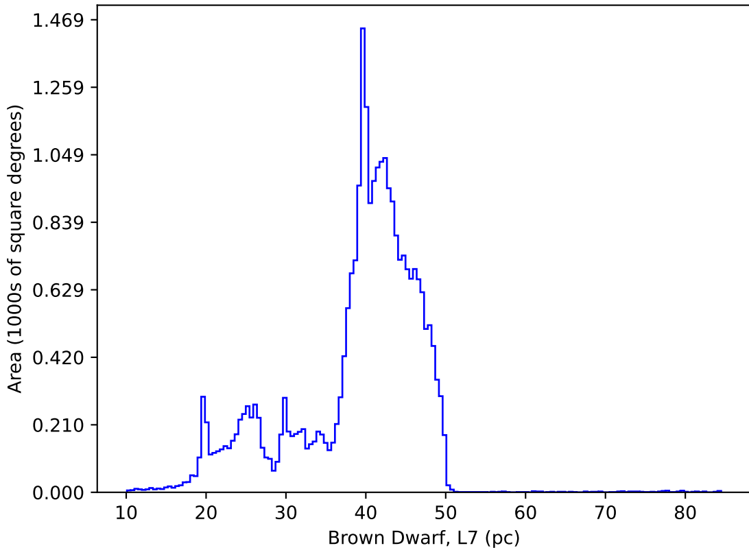
ddf_acor_sf15_lsf30_lsr20_v3.4_10yrs : Brown Dwarf, L7
