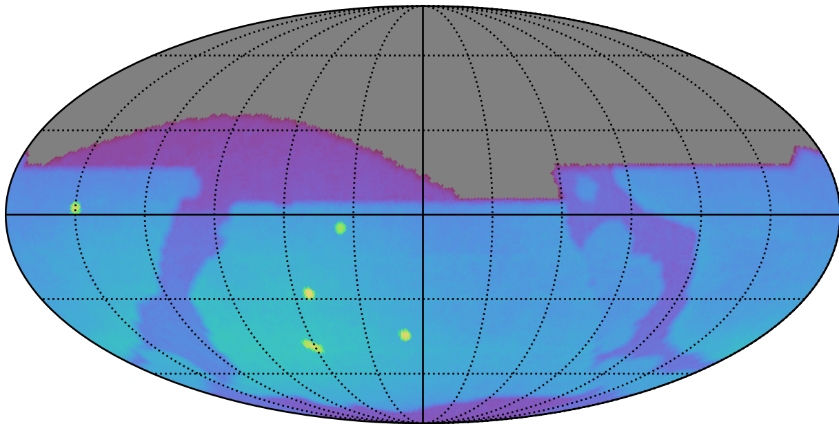
ddf_acor_sf15_lsf30_lsr20_v3.4_10yrs : Brown Dwarf, L4
