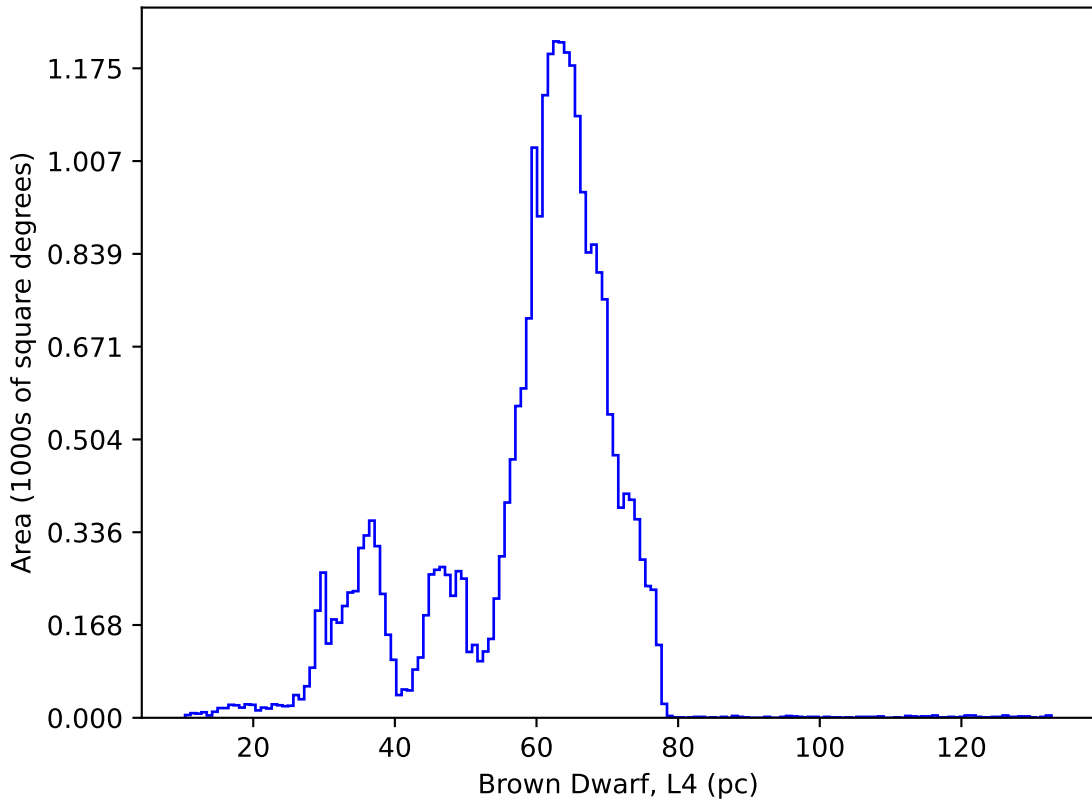
ddf_acor_sf15_lsf30_lsr20_v3.4_10yrs : Brown Dwarf, L4
