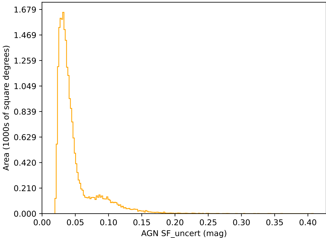
ddf_acor_sf15_lsf30_lsr20_v3.4_10yrs r band: AGN SF_uncert
