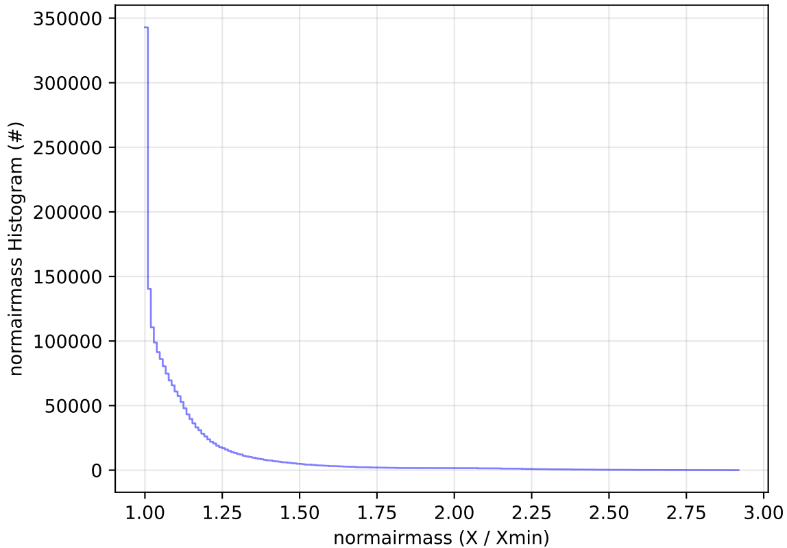
ddf_acor_sf15_lsf30_lsr20_v3.4_10yrs WFD all bands: normairmass Histogram
