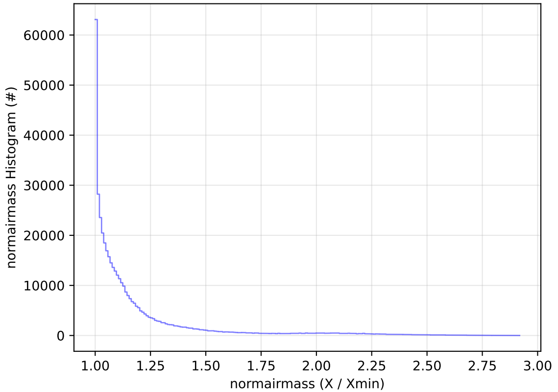
ddf_acor_sf15_lsf30_lsr20_v3.4_10yrs All sky z band: normairmass Histogram
