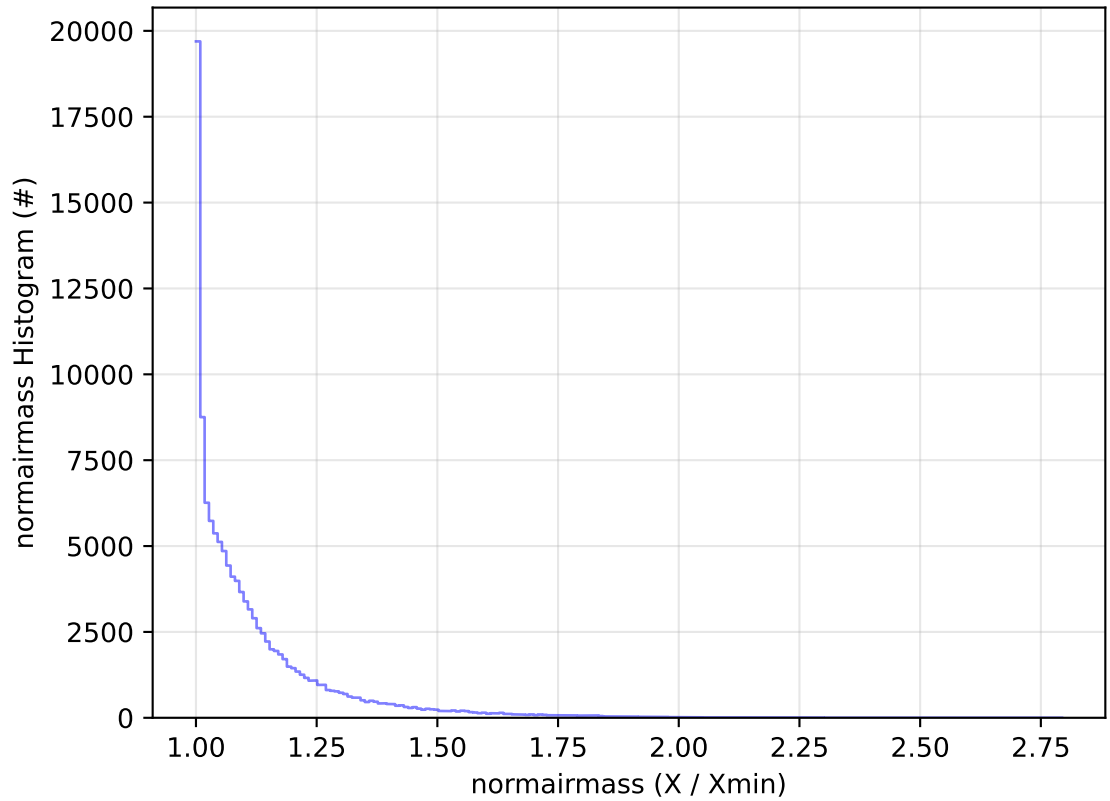
ddf_acor_sf15_lsf30_lsr20_v3.4_10yrs All sky u band: normairmass Histogram
