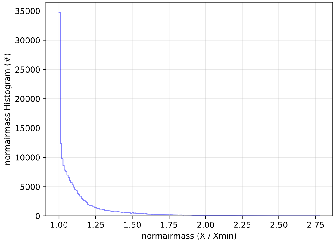
ddf_acor_sf15_lsf30_lsr20_v3.4_10yrs All sky g band: normairmass Histogram
