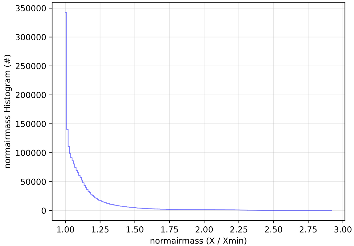
ddf_acor_sf15_lsf30_lsr20_v3.4_10yrs All sky all bands: normairmass Histogram
