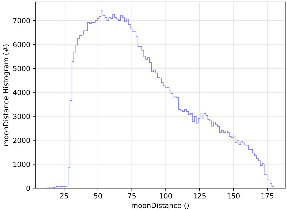
ddf_acor_sf15_Isf30_Isr20_v3.4_10yrs WFD z band: moonDistance Histogram
