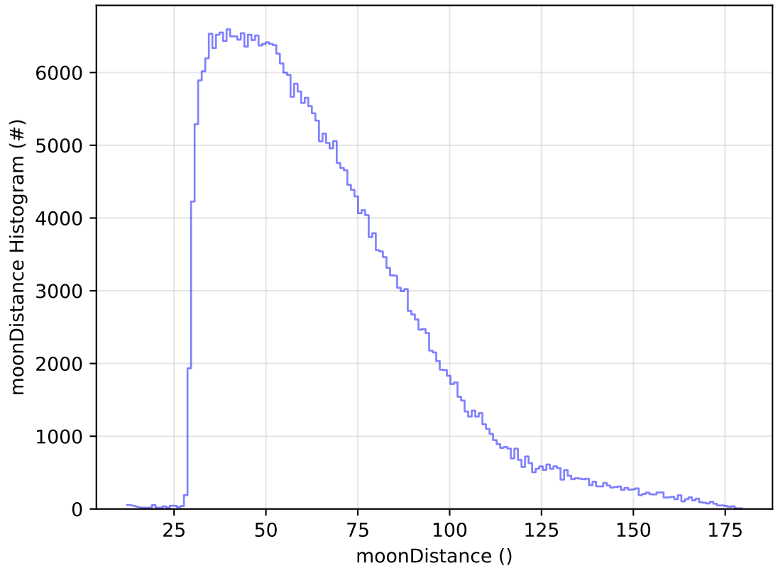
ddf_acor_sf15_Isf30_Isr20_v3.4_10yrs WFD y band: moonDistance Histogram
