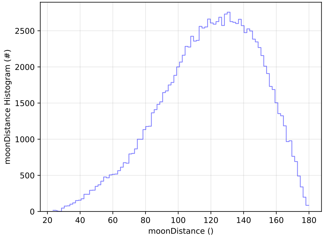
ddf_acor_sf15_lsf30_lsr20_v3.4_10yrs WFD u band: moonDistance Histogram
