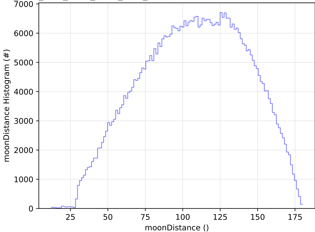
ddf_acor_sf15_lsf30_lsr20_v3.4_10yrs WFD r band: moonDistance Histogram
