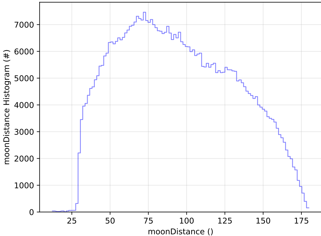
ddf_acor_sf15_lsf30_lsr20_v3.4_10yrs WFD i band: moonDistance Histogram
