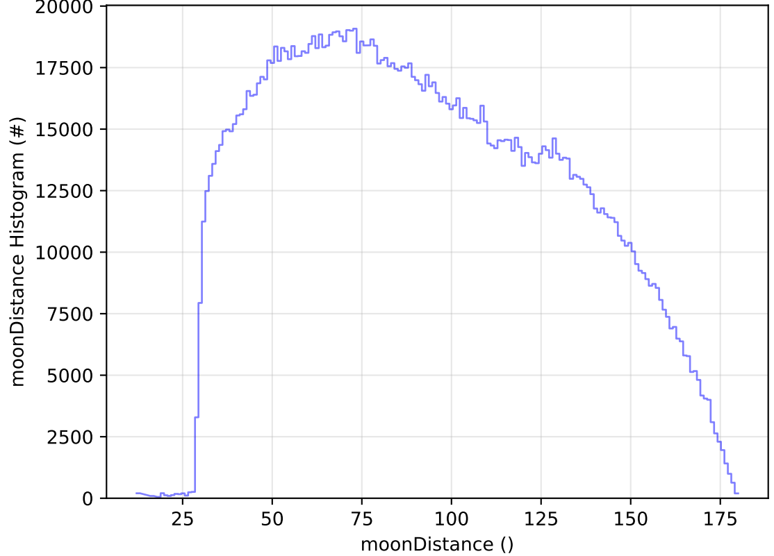
ddf_acor_sf15_lsf30_lsr20_v3.4_10yrs WFD all bands: moonDistance Histogram
