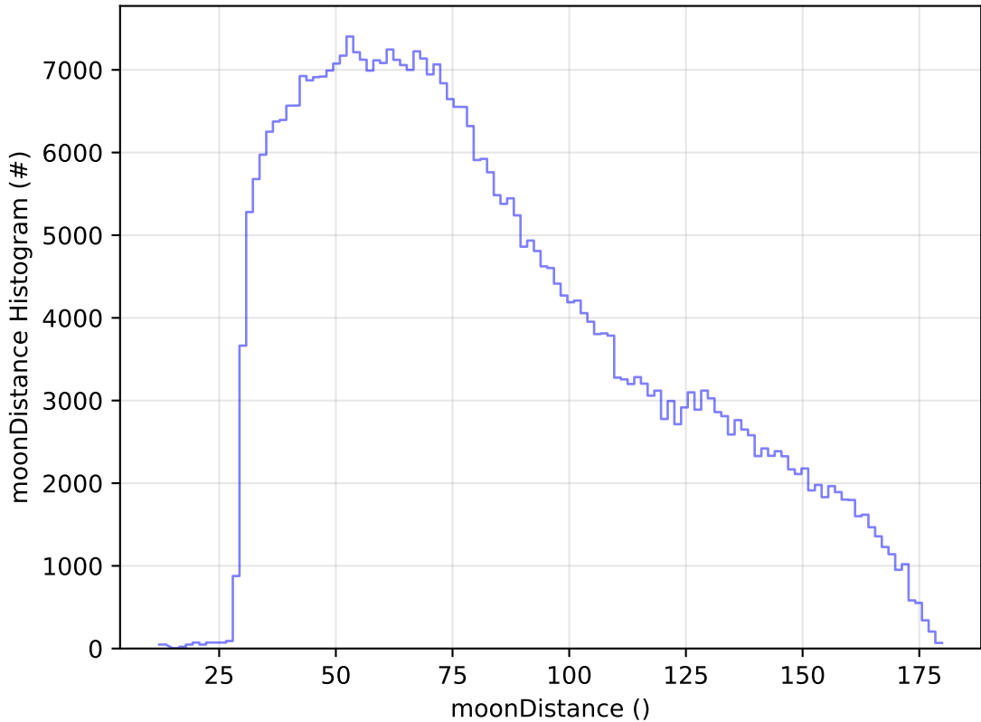
ddf_acor_sf15_lsf30_lsr20_v3.4_10yrs All sky z band: moonDistance Histogram
