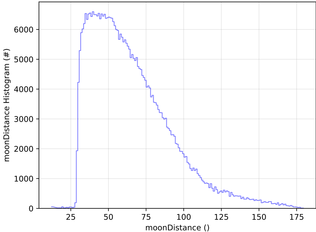
ddf_acor_sf15_lsf30_lsr20_v3.4_10yrs All sky y band: moonDistance Histogram
