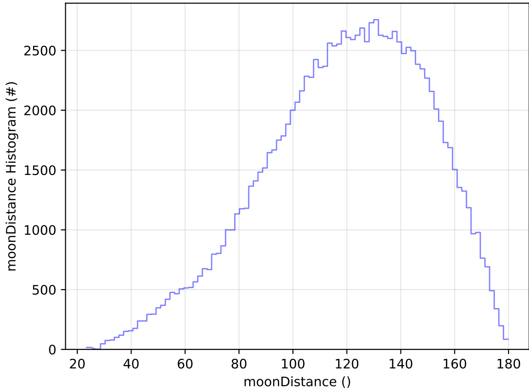
ddf_acor_sf15_lsf30_lsr20_v3.4_10yrs All sky u band: moonDistance Histogram
