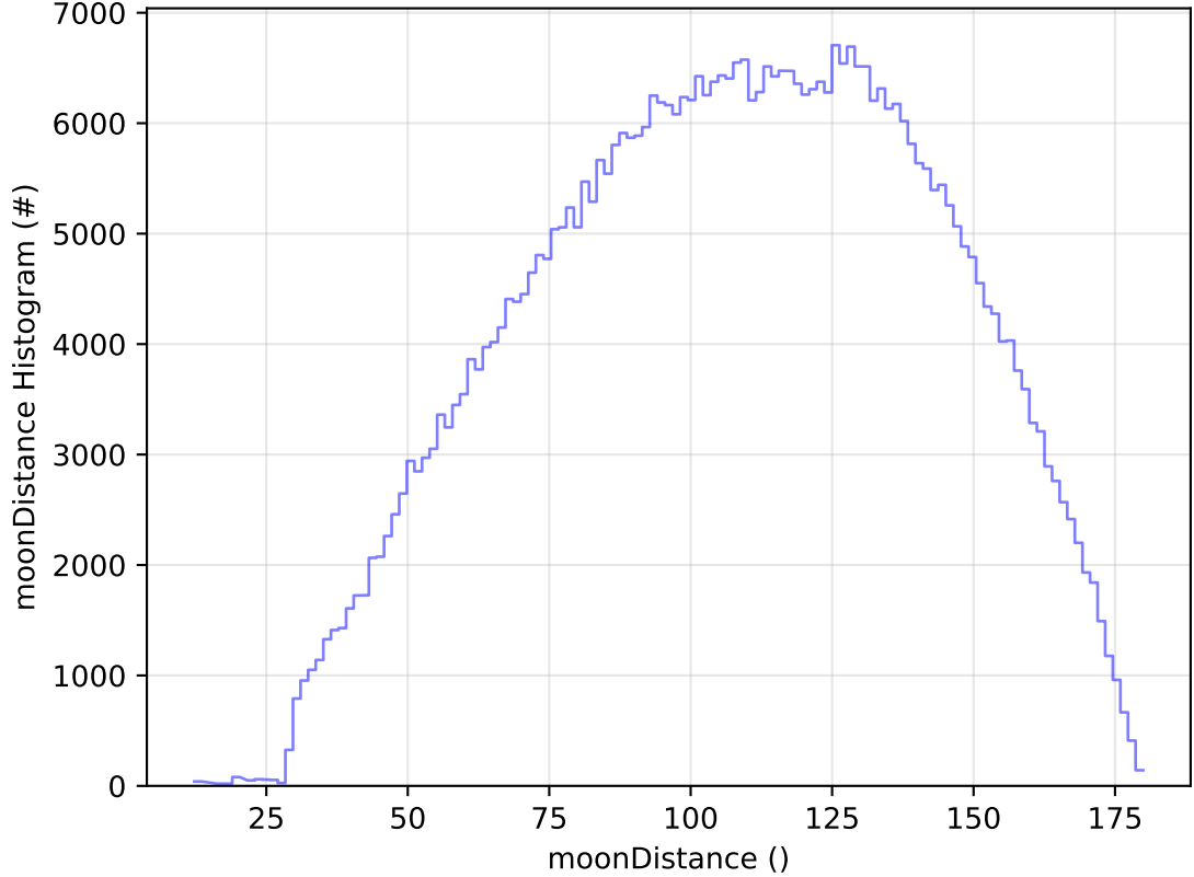
ddf_acor_sf15_lsf30_lsr20_v3.4_10yrs All sky r band: moonDistance Histogram
