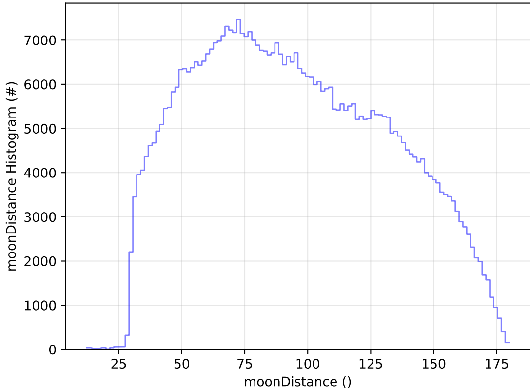
ddf_acor_sf15_lsf30_lsr20_v3.4_10yrs All sky i band: moonDistance Histogram
