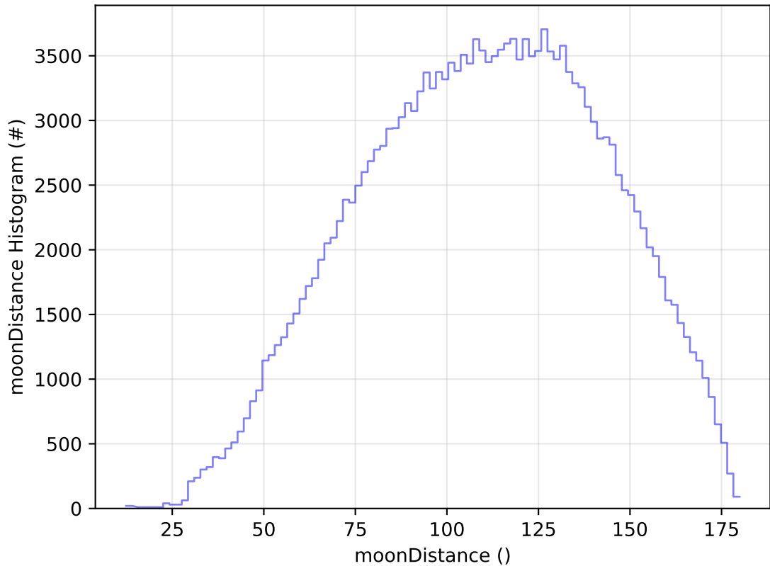
ddf_acor_sf15_lsf30_lsr20_v3.4_10yrs All sky g band: moonDistance Histogram
