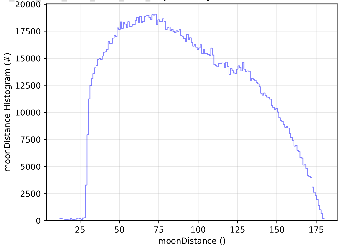
ddf_acor_sf15_lsf30_lsr20_v3.4_10yrs All sky all bands: moonDistance Histogram
