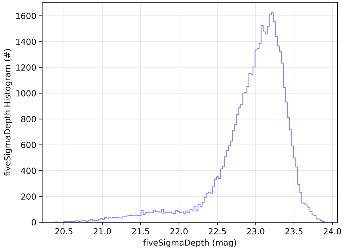
ddf_acor_sf15_lsf30_lsr20_v3.4_10yrs Yr 1 z band: fiveSigmaDepth Histogram
