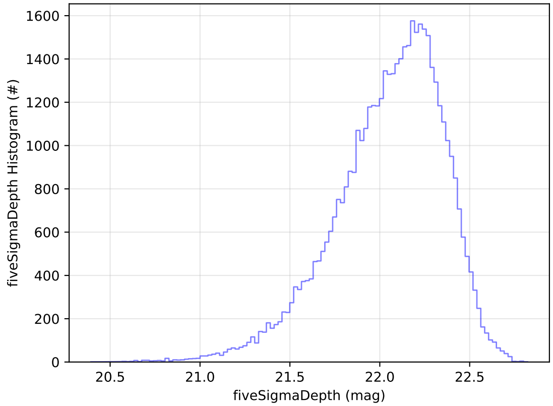
ddf_acor_sf15_lsf30_lsr20_v3.4_10yrs Yr 1 y band: fiveSigmaDepth Histogram
