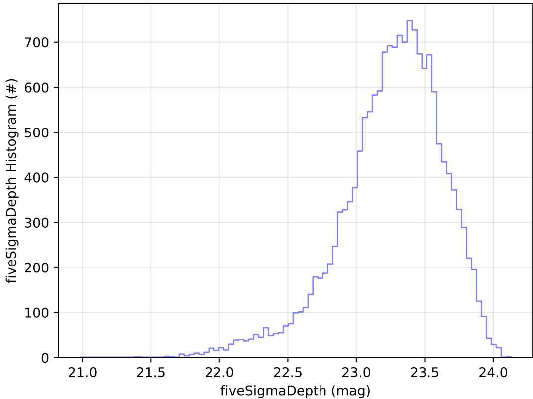
ddf_acor_sf15_lsf30_lsr20_v3.4_10yrs Yr 1 u band: fiveSigmaDepth Histogram
