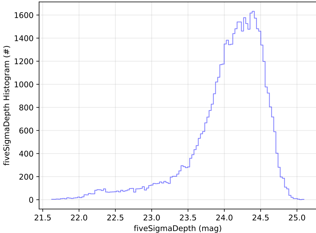
ddf_acor_sf15_lsf30_lsr20_v3.4_10yrs Yr 1 r band: fiveSigmaDepth Histogram
