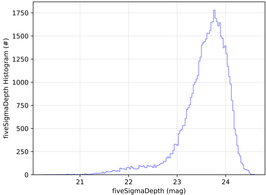
ddf_acor_sf15_lsf30_lsr20_v3.4_10yrs Yr 1 i band: fiveSigmaDepth Histogram
