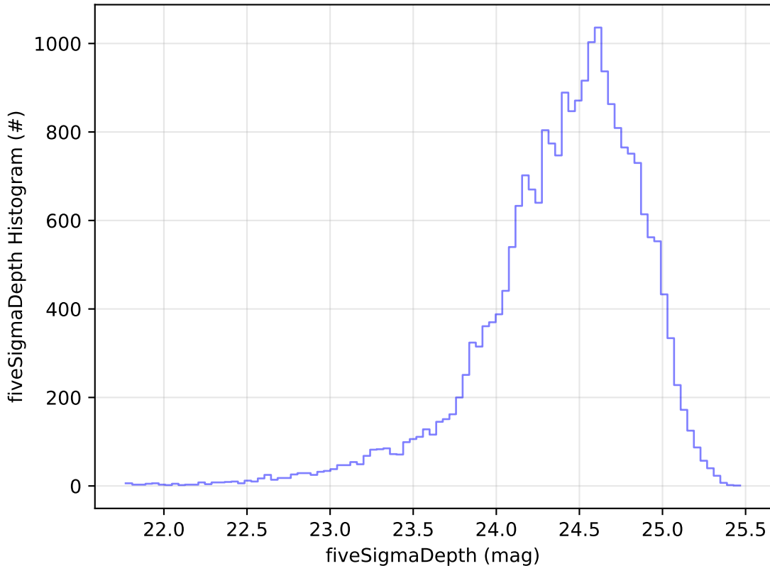
ddf_acor_sf15_lsf30_lsr20_v3.4_10yrs Yr 1 g band: fiveSigmaDepth Histogram
