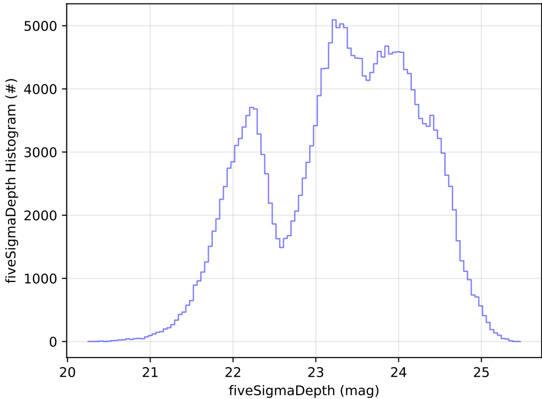
ddf_acor_sf15_lsf30_lsr20_v3.4_10yrs Yr 1 all bands: fiveSigmaDepth Histogram
