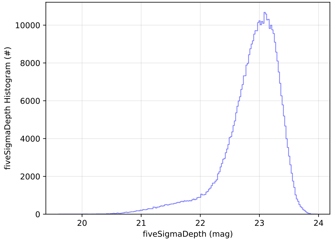
ddf_acor_sf15_lsf30_lsr20_v3.4_10yrs WFD z band: fiveSigmaDepth Histogram
