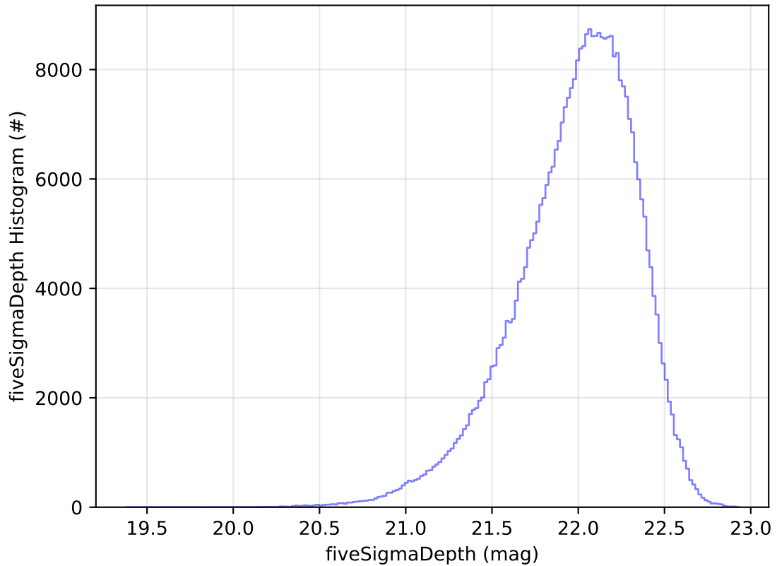
ddf_acor_sf15_lsf30_lsr20_v3.4_10yrs WFD y band: fiveSigmaDepth Histogram
