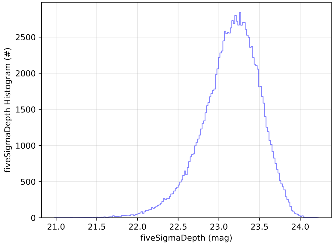
ddf_acor_sf15_lsf30_lsr20_v3.4_10yrs WFD u band: fiveSigmaDepth Histogram
