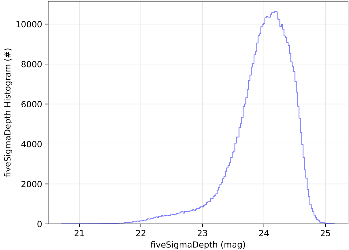
ddf_acor_sf15_lsf30_lsr20_v3.4_10yrs WFD r band: fiveSigmaDepth Histogram
