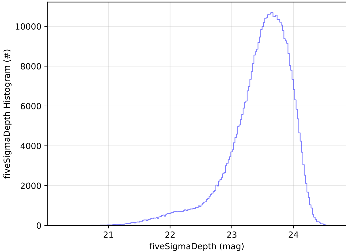
ddf_acor_sf15_lsf30_lsr20_v3.4_10yrs WFD i band: fiveSigmaDepth Histogram
