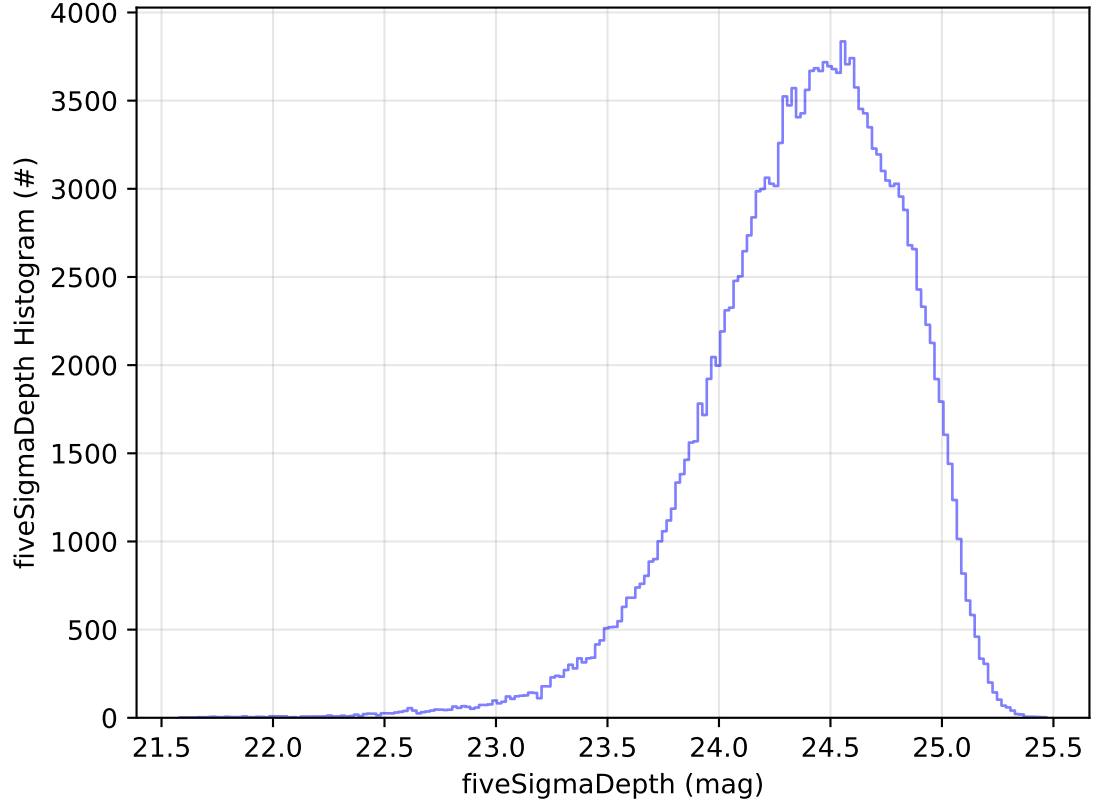
ddf_acor_sf15_lsf30_lsr20_v3.4_10yrs WFD g band: fiveSigmaDepth Histogram
