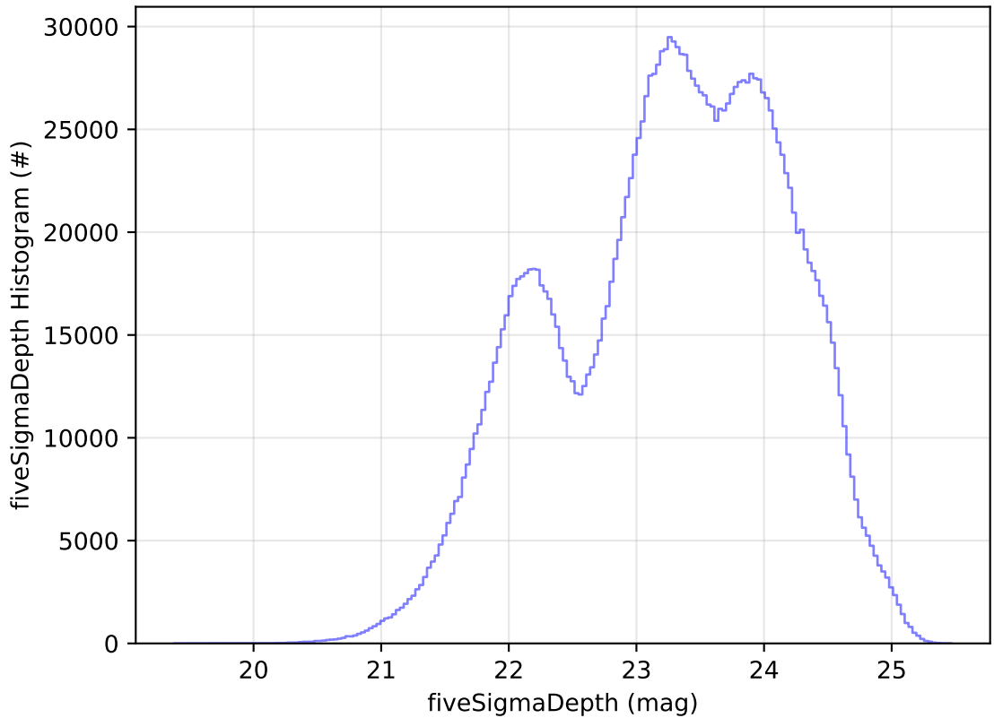
ddf_acor_sf15_lsf30_lsr20_v3.4_10yrs WFD all bands: fiveSigmaDepth Histogram
