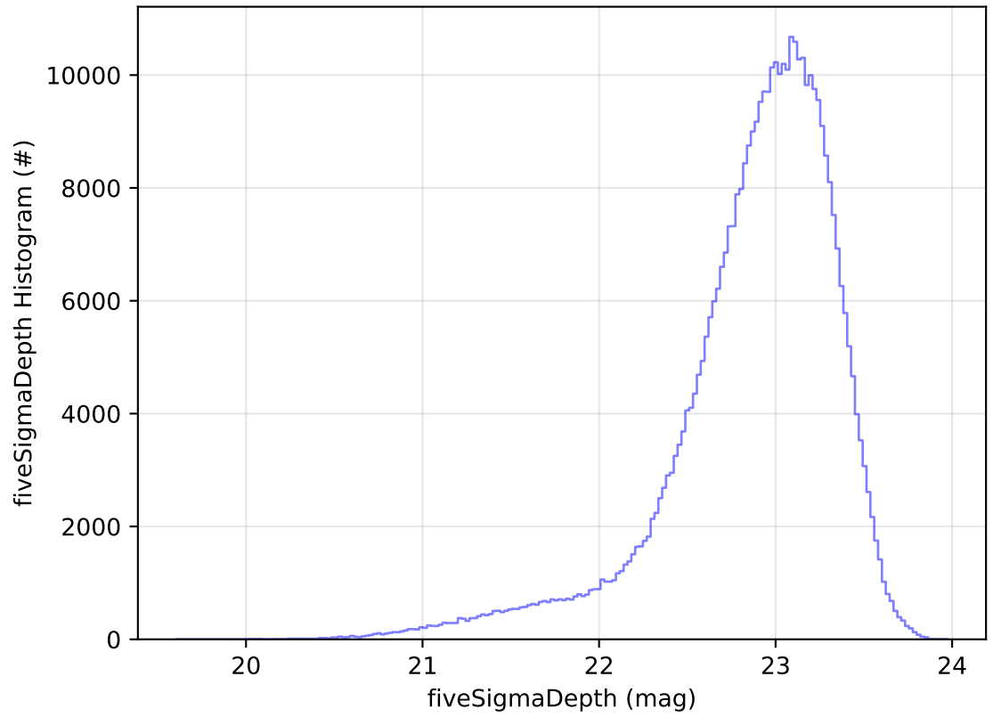
ddf_acor_sf15_lsf30_lsr20_v3.4_10yrs All sky z band: fiveSigmaDepth Histogram
