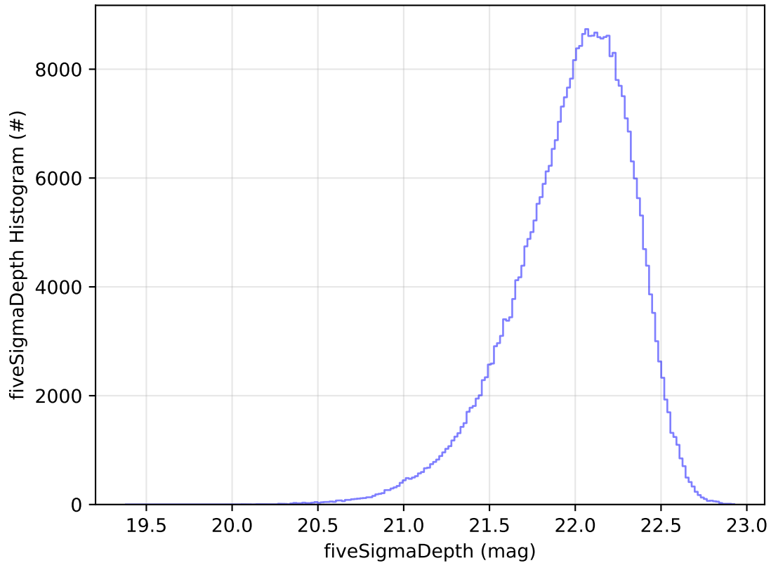
ddf_acor_sf15_lsf30_lsr20_v3.4_10yrs All sky y band: fiveSigmaDepth Histogram
