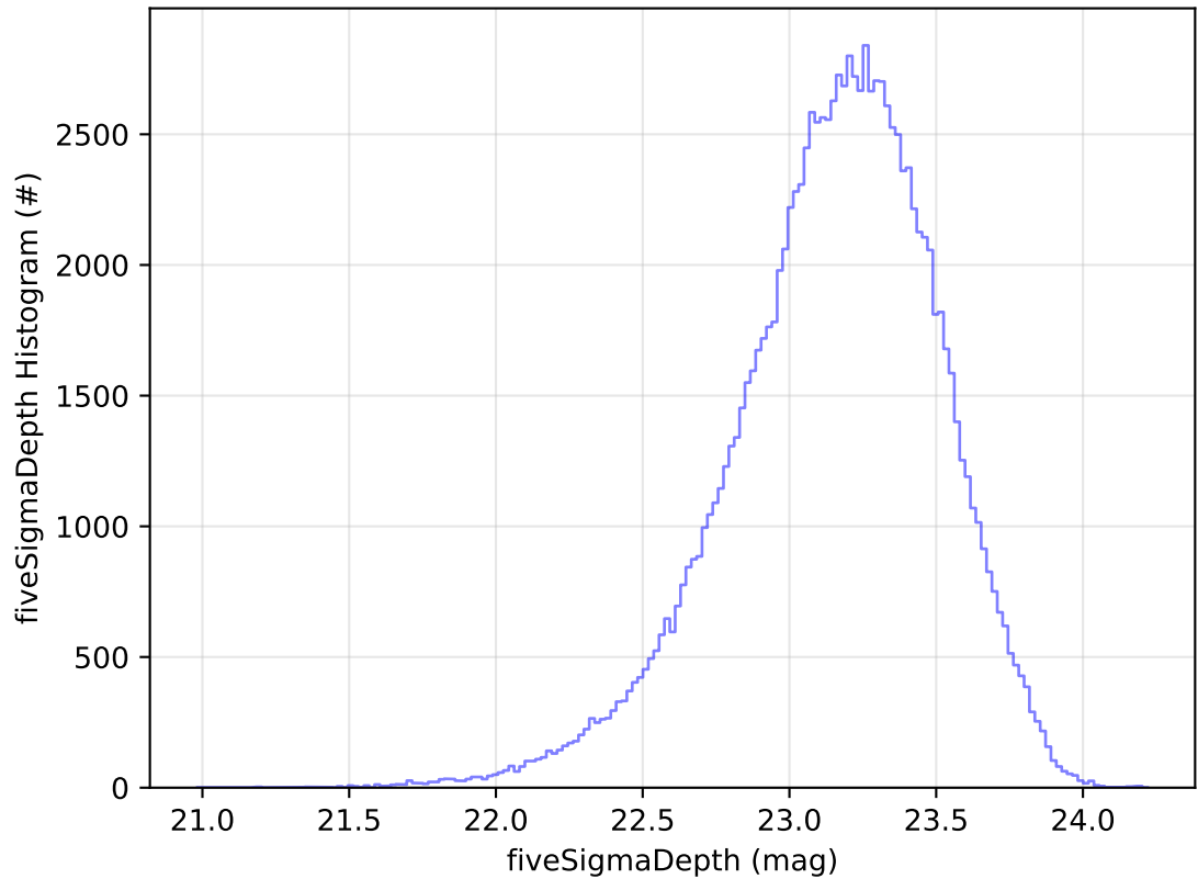
ddf_acor_sf15_lsf30_lsr20_v3.4_10yrs All sky u band: fiveSigmaDepth Histogram
