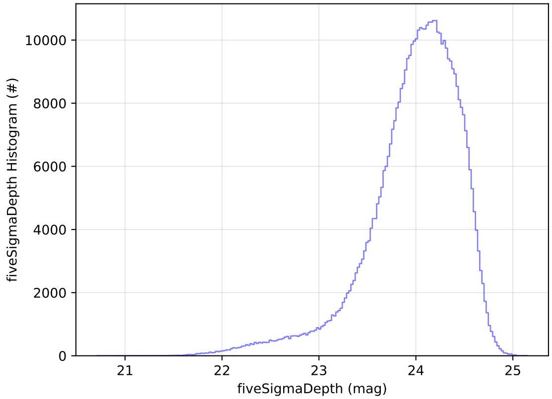
ddf_acor_sf15_lsf30_lsr20_v3.4_10yrs All sky r band: fiveSigmaDepth Histogram
