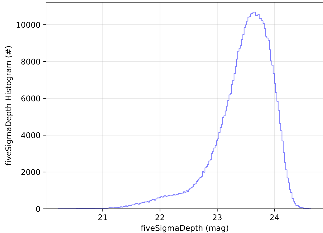
ddf_acor_sf15_lsf30_lsr20_v3.4_10yrs All sky i band: fiveSigmaDepth Histogram
