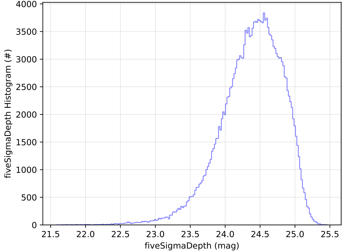
ddf_acor_sf15_lsf30_lsr20_v3.4_10yrs All sky g band: fiveSigmaDepth Histogram
